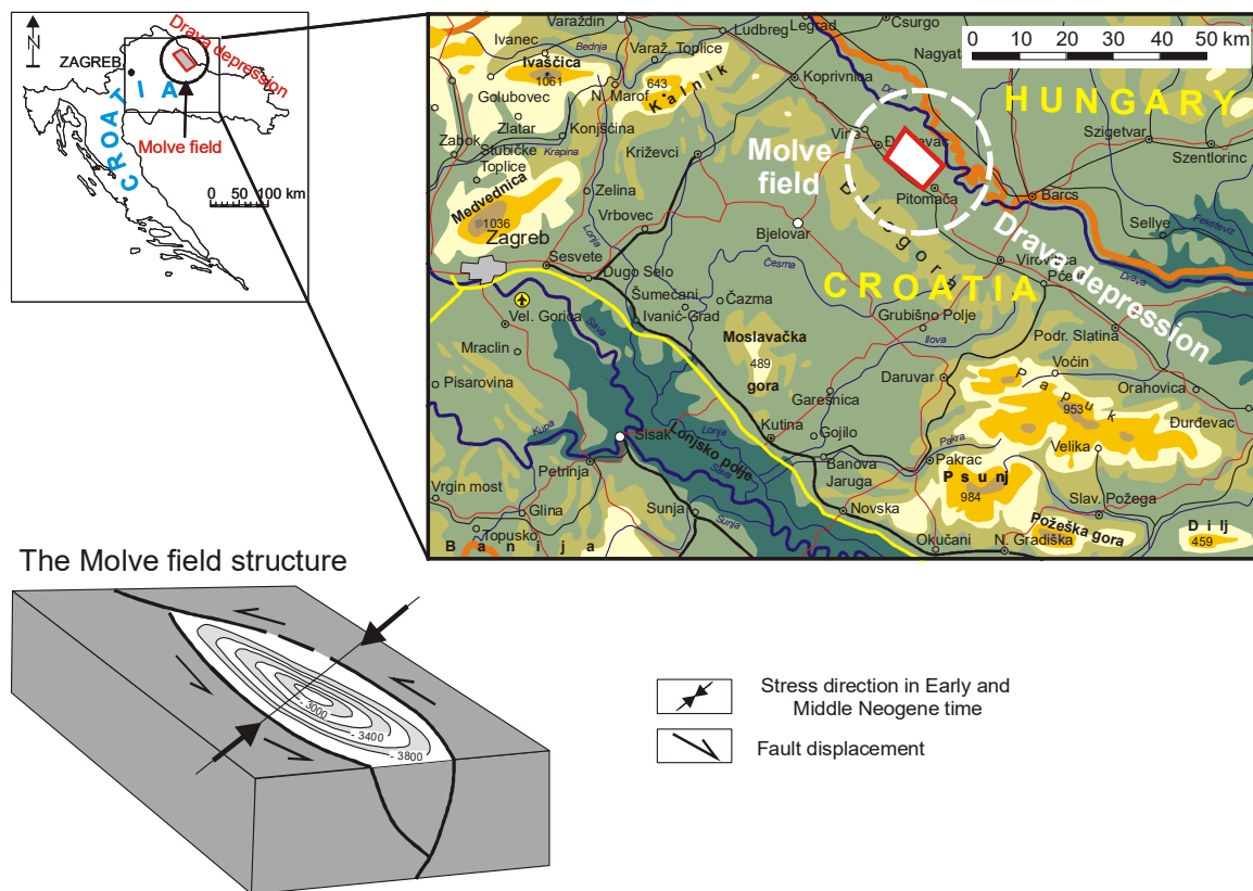
Figure 13. Geographical location of the Molve structure [44].
